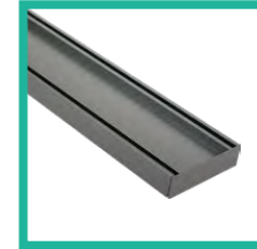
Gunmetal Slimline Tile Insert 26 (STI26-GM-3 | STI26-GM-5.6) 100mm x 26mm x 3000mm 100mm x 26mm x 5600mm
