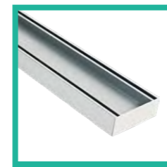
Silver Tile Insert Plus (TIP35-S-3 | TIP35-S-5.6) 100mm x 35mm x 3000mm 100mm x 35mm x 5600mm
