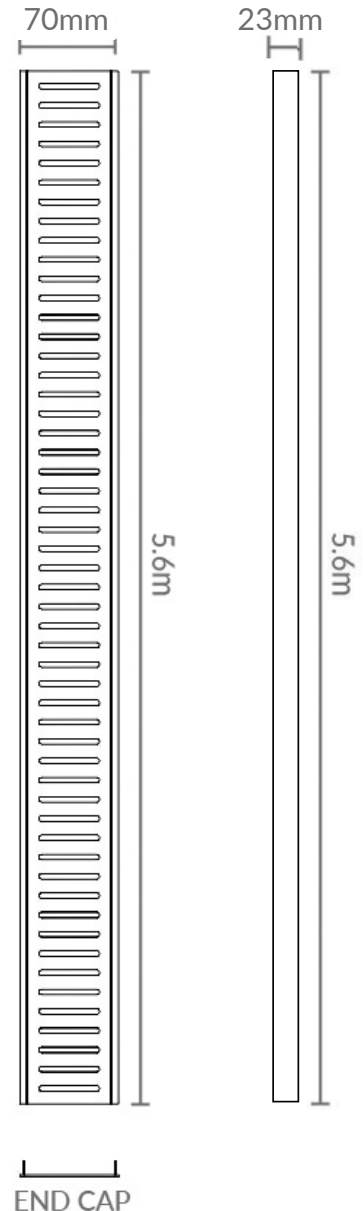
TOP VIEW
